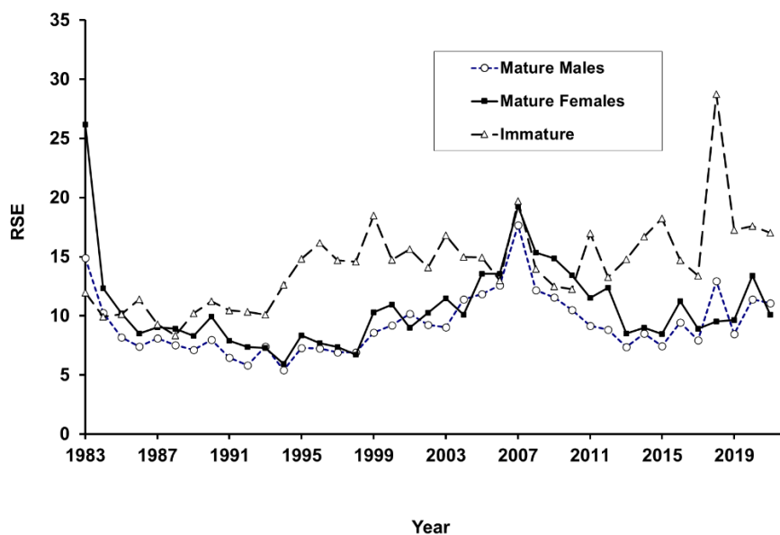
Figure 4. Relative standard error ( RSE = \{SE / \text{Mean}\} * 100 ) of the annual CPUE (number/lift) for mature male, mature female and immature (sexes combined) lake trout caught with USGS-NYSDEC gill nets set in U.S. waters of Lake Ontario during September 1983-2021. RSE increases after 1993 are in part due a reduction in the number of sites sampled declining from 17 to 14 in 1994. Reduced effort in 2018 and 2020 (only 8 sites fished in each year) contributed to the in RSE for those years.
