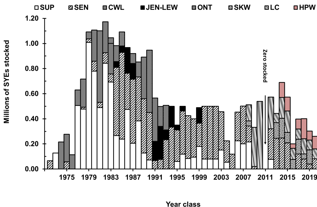
Figure 2. Total spring yearling equivalents (SYE) for lake trout strains stocked in U.S. waters of Lake Ontario for the 1972 – 2020 year-classes. Strain descriptions for ONT (Lake Ontario), JEN-LEW (Jenny-Lewis Lakes), CWL (Clearwater Lake), SEN (Seneca Lake), LC (Lake Champlain), SUP (Lake Superior), SKW (Lake Superior Klondikes), HPW (Lake Huron-Parry Sound) appear in Appendix 1. For year-classes beginning in 2006, SUP refers to Lake Superior the lean strains SAW (Lake Superior, Apostle Islands) and STW (Lake Superior, Traverse Islands) other than the Superior Marquette Domestics stocked prior to that time. SYE = 1 spring yearling or 2.4 fall fingerlings (Elrod et al. 1988). No lake trout from the 2011 year-class were stocked in 2012.
