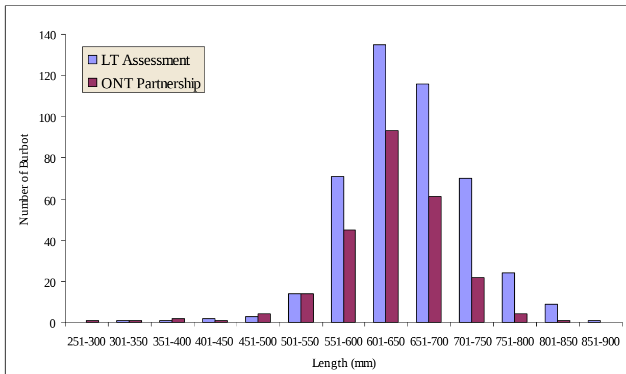
Figure 3.5. Length distribution of burbot collected from all jurisdictions in the summer gill net assessment, 2003 (n = 447), and the OMNR Partnership Index Fishing Program, 2003 (n = 249).
