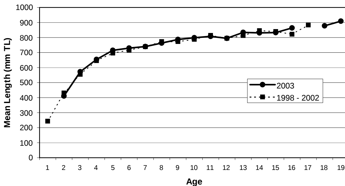
Figure 1.7. Mean length-at-age of lake trout collected in gill nets from the eastern basin of Lake Erie, August, 2003. The previous 5-year average (1998 – 2002) from New York are shown for current growth rate comparison.
