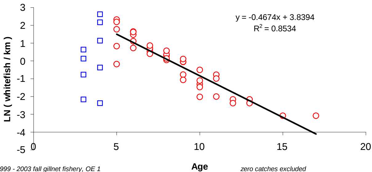
Figure 2.4. Catch curve for lake whitefish using Ontario fall large mesh gill net CPUE (# / km) from 1999 to 2003. Open circles represent fully recruited ages used in regression. Squares indicate partial recruitment to the gear. Z = -0.4674 ; Survival = 63%
