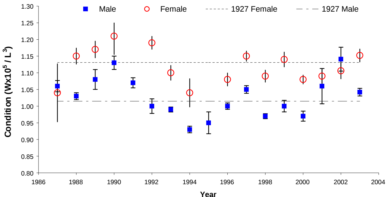
Figure 2.8. Mean condition factor of lake whitefish by sex from 1987 to 2003 with one standard error. Data include whitefish ages 4 and older collected from commercial fish and Partnership index samples from October to December. Spent and ripe whitefish were excluded. Historic mean condition (1927 – 1929) presented as dashed lines, calculated from Van Oosten and Hile (1947).
