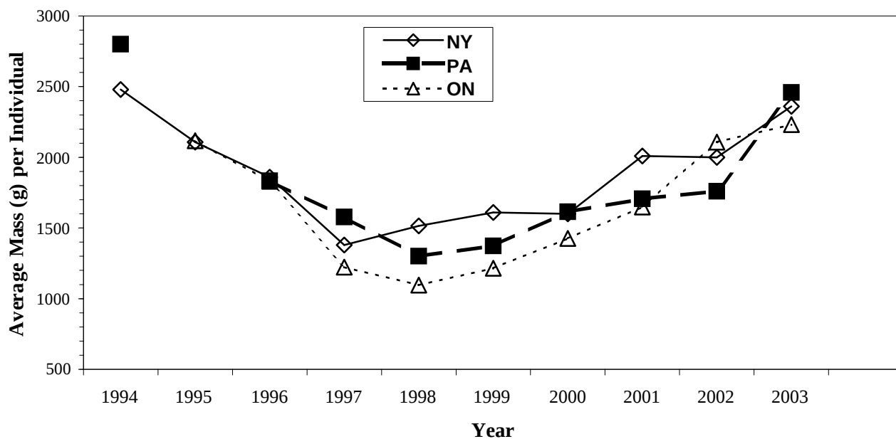
Figure 3.3. Average mass (g) per individual burbot from summer gill net assessment by jurisdiction, 1994 - 2003.
