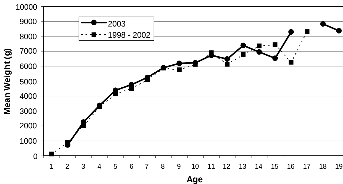
Figure 1.8. Mean weight-at-age of lake trout collected in gill nets from the eastern basin of Lake Erie, August, 2003. The previous 5-year average (1998 – 2002) from New York are shown for current growth rate comparison.
