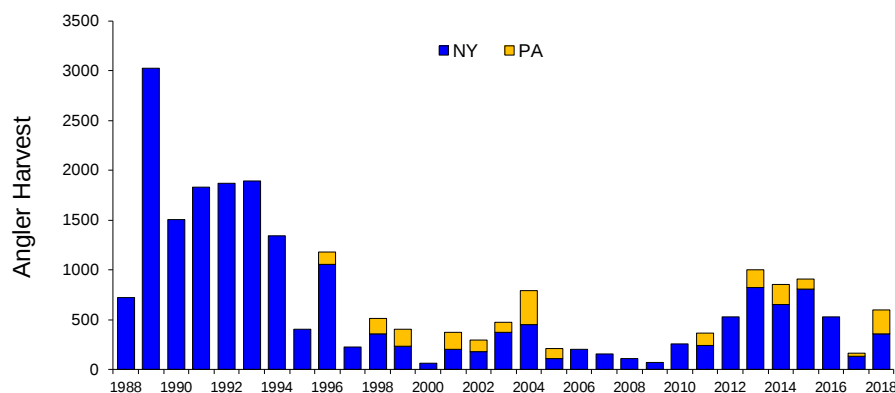
FIGURE 1.6. Estimated Lake Trout harvest by recreational anglers in the New York and Pennsylvania waters of Lake Erie, 1988-2018.
