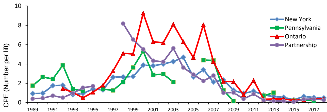
FIGURE 1.8. Burbot CPE (number per lift) by basin from the Interagency Coldwater Assessment and Ontario Partnership Surveys bottom set nets.
