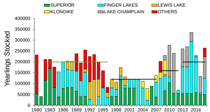
Lake Trout Stocking 1980-2018
