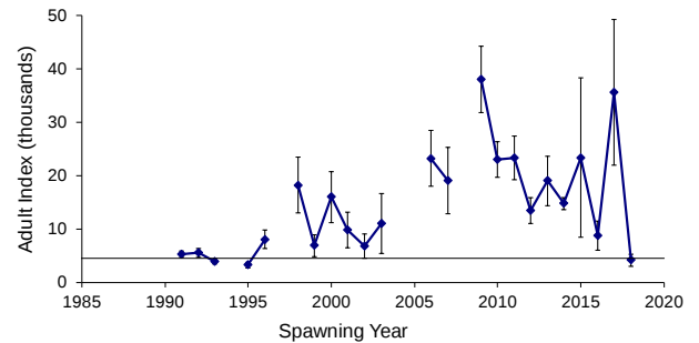
Sea Lamprey Adult Index
