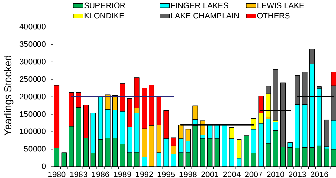
FIGURE 4.2. Lake Trout (in yearling equivalents) stocked by all jurisdictions in Lake Erie, 1980-2018, by strain. Stocking goals through time are shown by black lines dark lines; the current stocking goal is 200,000 yearlings per year. Superior includes Superior, Apostle Island, Traverse Island, Slate Island, and Michipicoten strains; Others include Clearwater Lake, Lake Ontario, Lake Erie, and Lake Manitou strains. 1 fall fingerling = 0.41 yearling equivalents.
