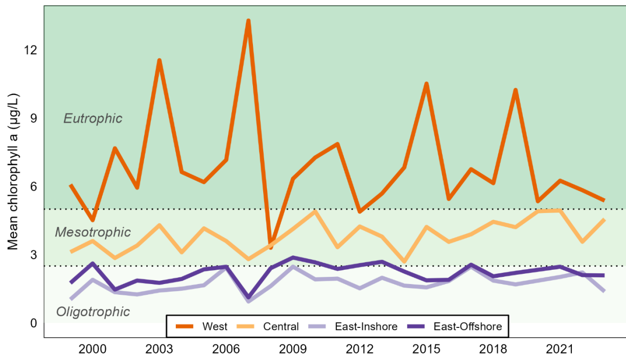
Figure 1.0.4: Mean chlorophyll a concentration (µg/L), weighted by month, for each basin in Lake Erie, 1999–2023. The East Basin is separated into nearshore and offshore. Shaded areas represent trophic class ranges.
