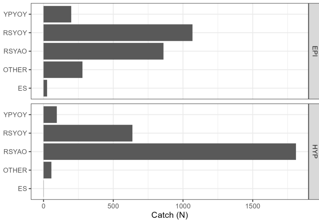
Figure 3.0.9: Total midwater trawl catch from epilimnetic (EPI, upper panel) and hypolimnetic (HYP, lower panel) tows across the Canadian waters and a portion of U.S. waters of the Central Basin, including species groups age-0 Rainbow Smelt (RSYOY), age-1+ Rainbow Smelt (RSYAO), Emerald Shiner (ES), age-0 Yellow Perch, and other species (OTHER).
