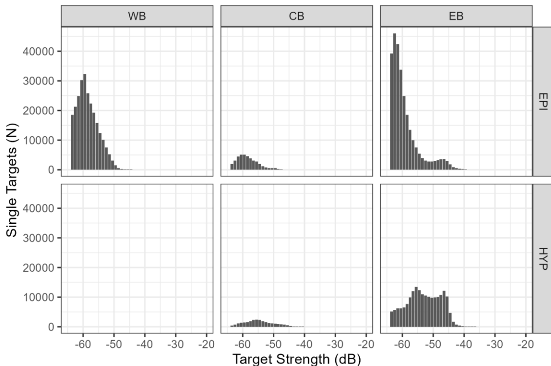
Figure 3.0.4: Target strength distributions of single targets by layer and across basins. Target strength is a measure of echo intensity that is relative to fish size. Single targets are individual echoes produced by fish encountered in the acoustic beam. In general, age-0 fishes are < -55 dB while age-1+ fishes are > -55 dB.
