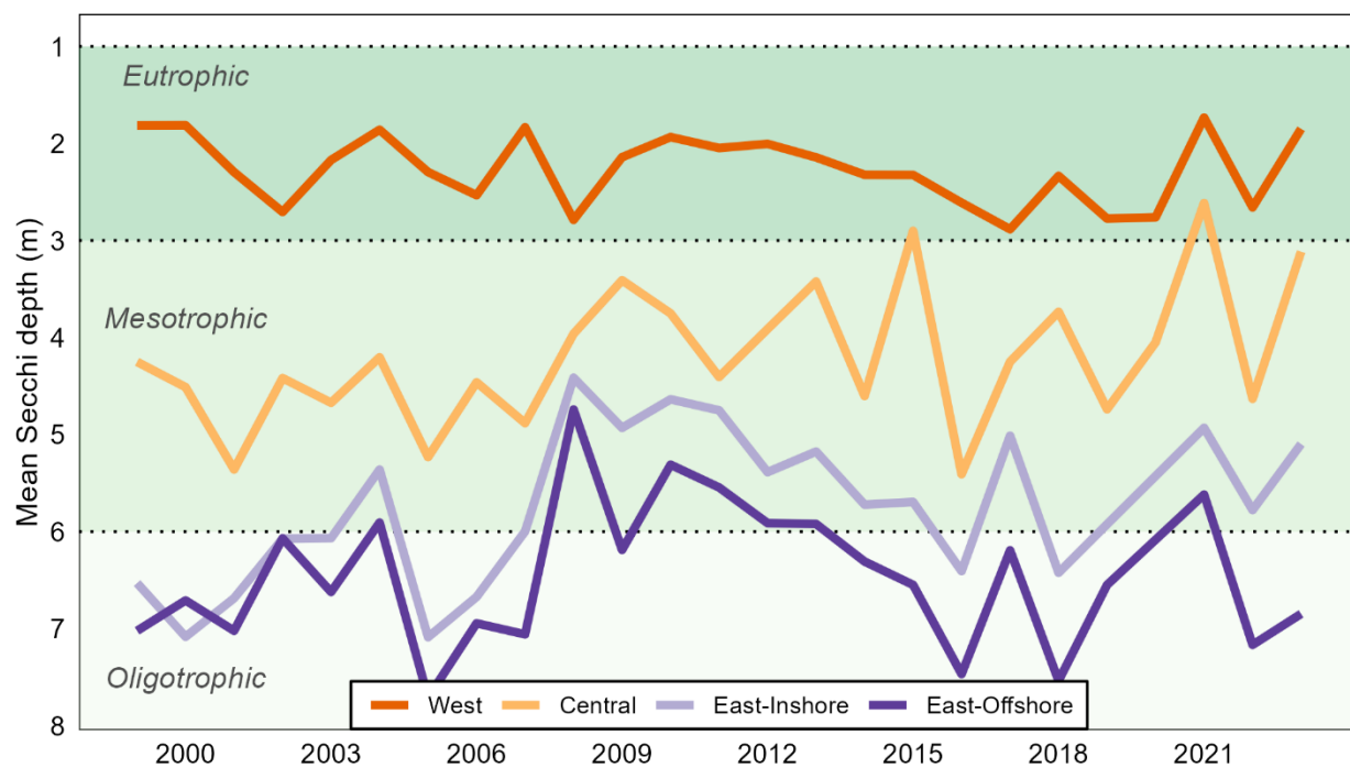
Figure 1.0.6: Mean summer (June–August) Secchi depth (m), weighted by month in each basin of Lake Erie, 1999–2023. The East Basin is separated into inshore and offshore. Shaded areas represent the trophic class ranges.
