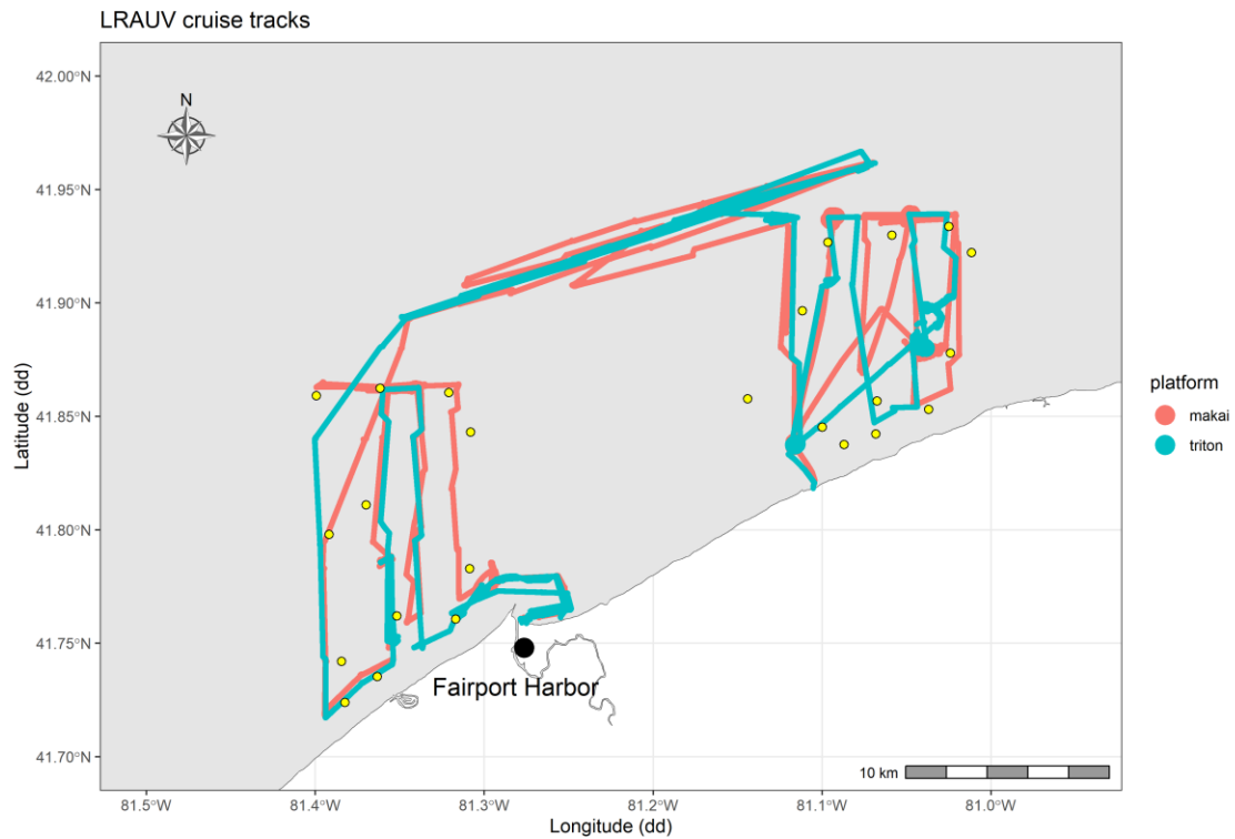
Figure 3.0.13: Long-range autonomous underwater vehicle (LRAUV) cruise tracks near Fairport Harbor, Ohio between September 9–17, 2023. The Triton (blue) collected upward and downward looking hydroacoustic data to evaluate near surface and near bottom biases. The Makai (red) collected eDNA samples with the goal of remotely characterizing fish community compositions. ODNr trawl locations (24) are indicated by yellow points circled in black.
