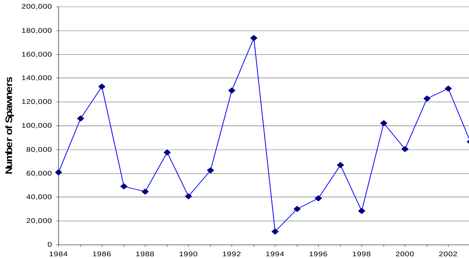
Fig. 4. Trend of spawner abundance for Lake Superior, 1984-2003.
