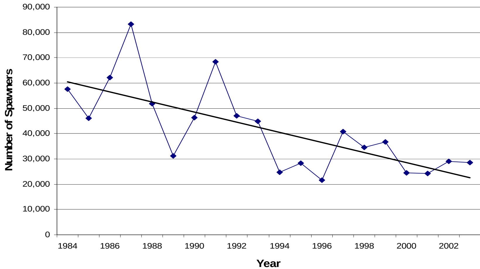
Fig 8. Trendline of the linear regression of spawner abundance for Lake Ontario, 1984-2003.
